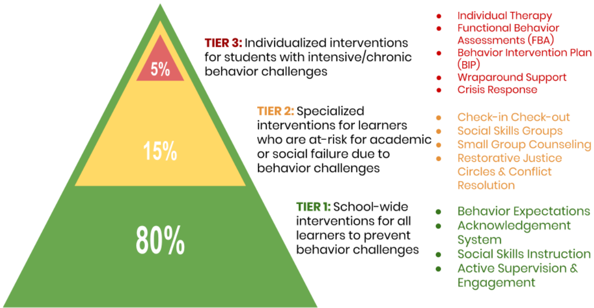
Figure 2.9: MTSS Model
