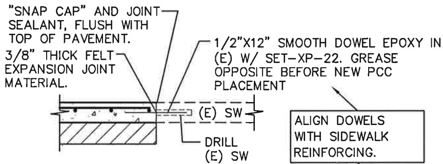
CONNECTION TO (E) CONCRETE
