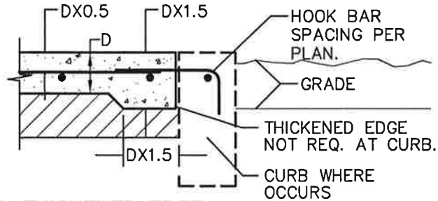
TYPICAL THICKENED EDGE
