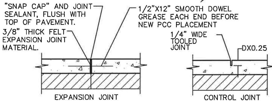
TYPICAL JOINTS
