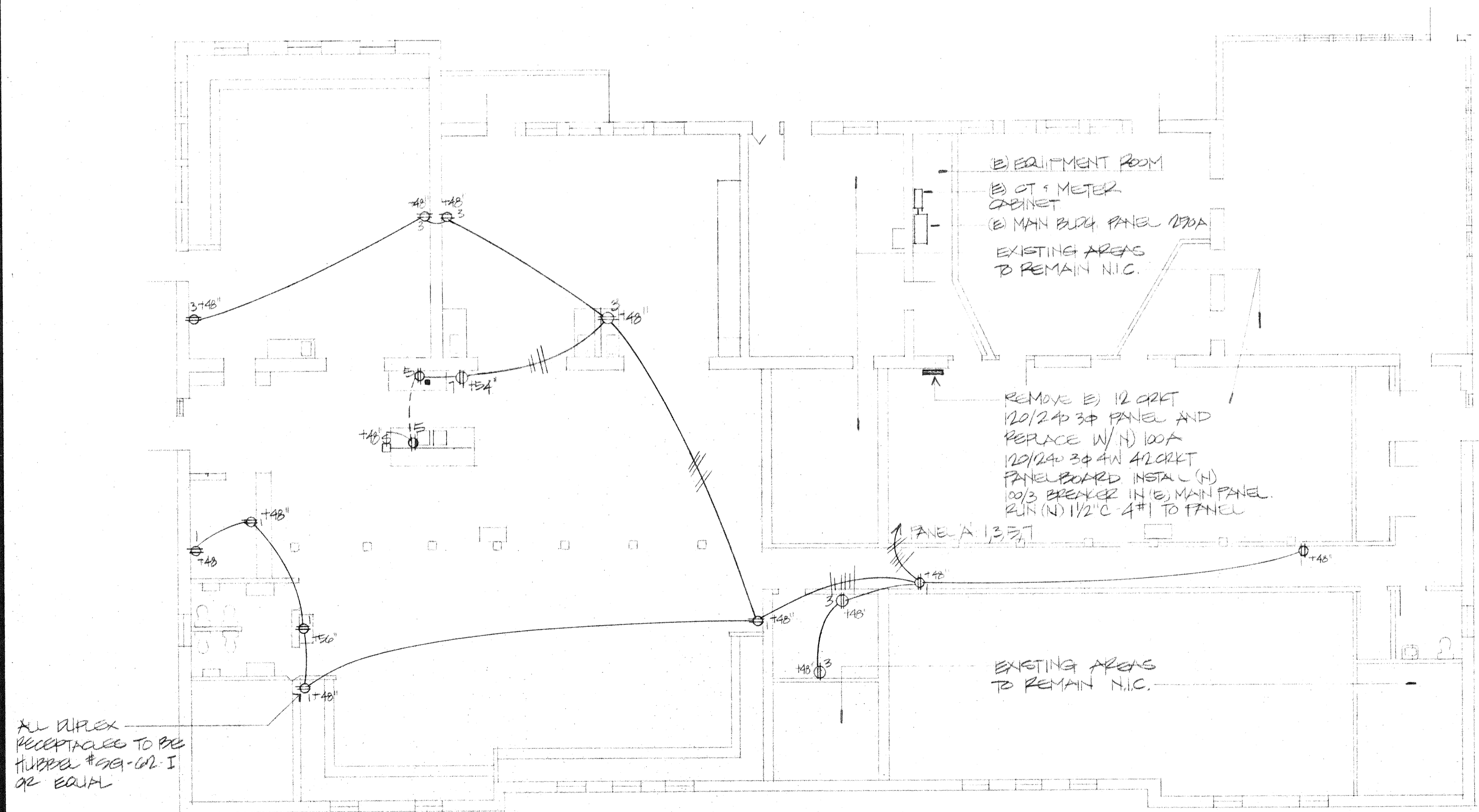
FLOOR PLAN - POWER AND SIGNAL SCALE: 1/8" = 1'-0"
